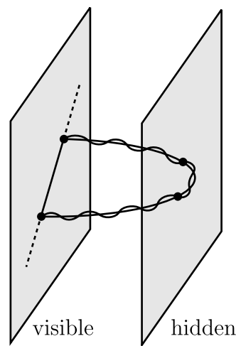
Figure 1: The leading diagram that contributes to SUSY-breaking scalar masses in the models considered in this paper. The bulk line is a gaugino propagator with two mass insertions on the hidden brane.
